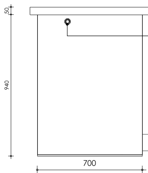
Left-side view
