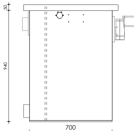
Right-side view
